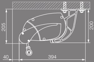
Top fix (with optional Vario-valance)
