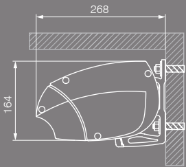
Wall fix
