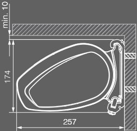
Wall fix
